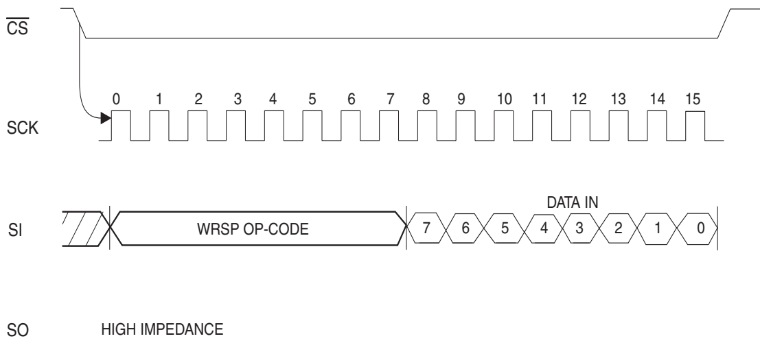
Figure 5-5. WRSR Timing
